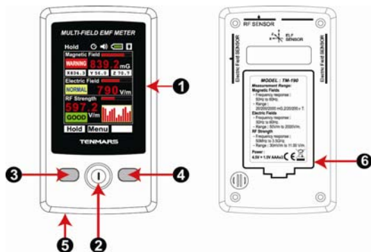
Fig. 2 Instrument description:
