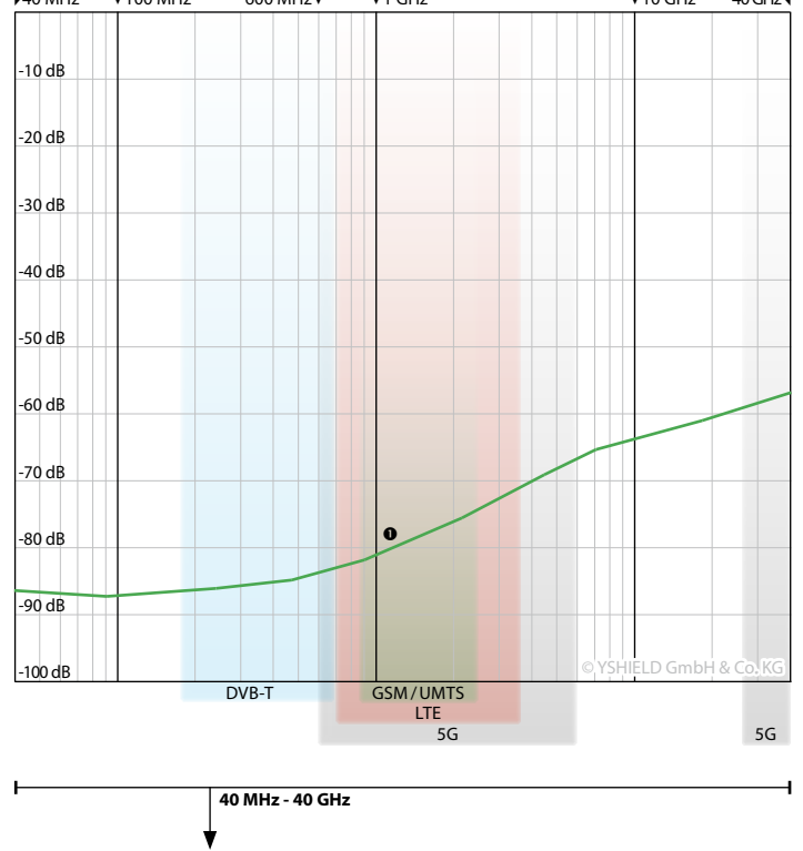
Screening attenuation Shielding fleece HNV80 ● Single layer ● Double layer ● Three layer
